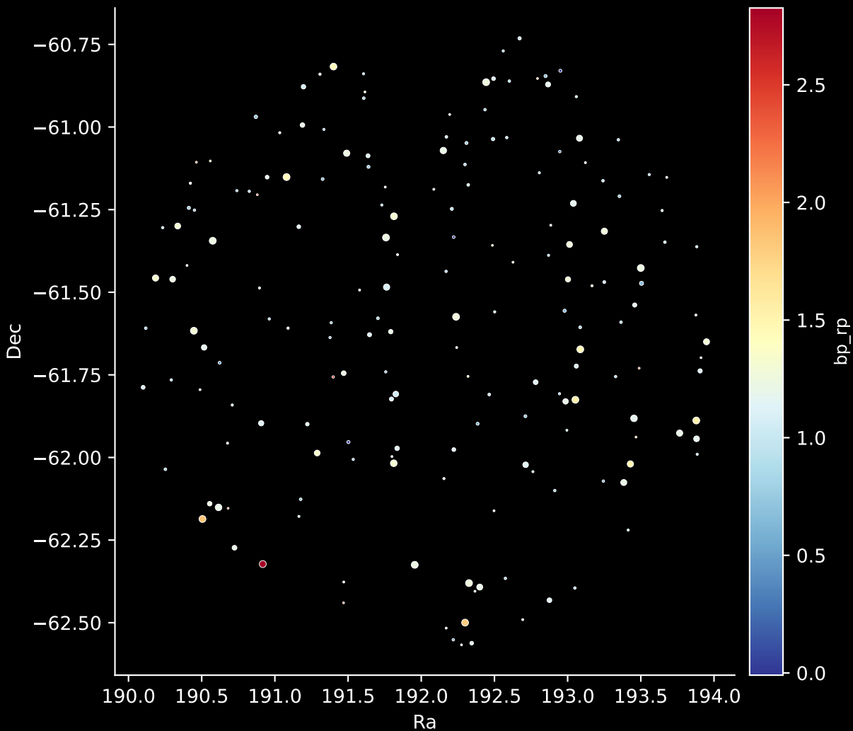
APOGEE DR17 Field: [271-29-O_TESS] Stars: 179
