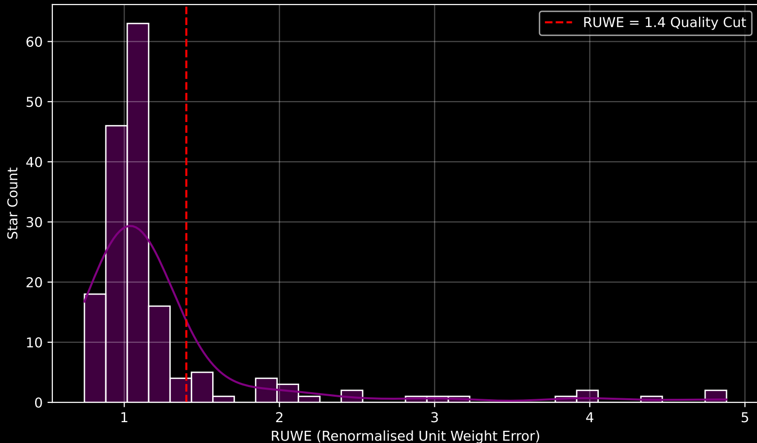
GAPOGEE DR17 Field [271-29-O_TESS] RUWE Distribution (n= 172)
