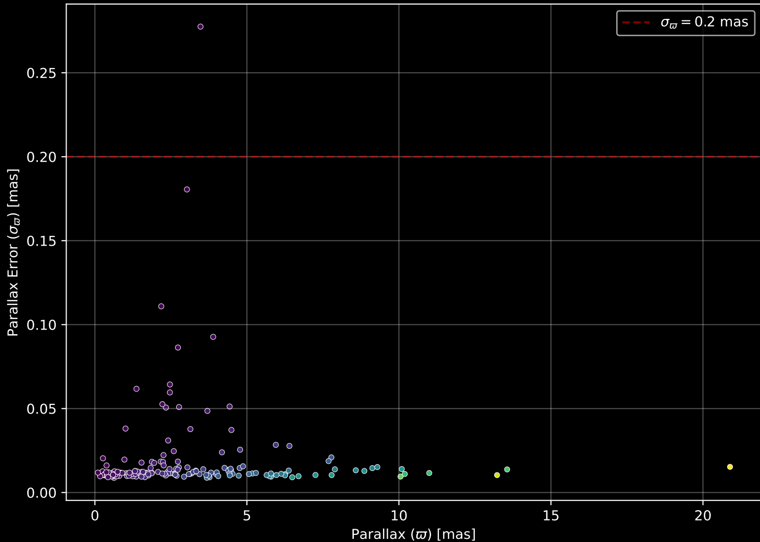
APOGEE DR17 Field: [271-29-O_TESS] Parallax Quality (n= 179)
