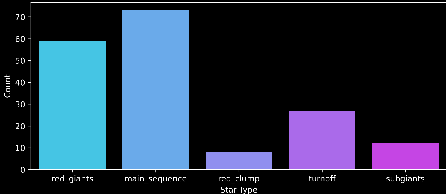
APOGEE DR17 Field: [271-29-O_TESS] Count plot of Star Type
