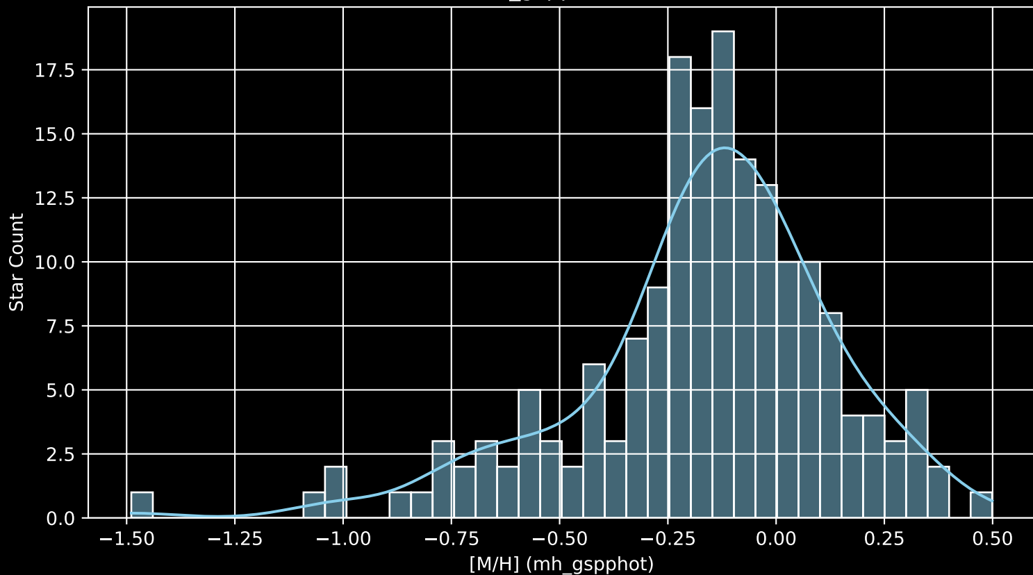
APOGEE DR17 Field: [271-29-O_TESS [M/H] (mh_gspphot) (n= 178)
