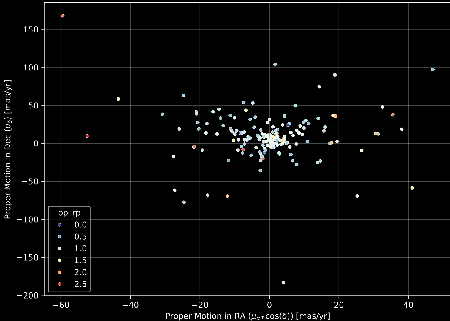
APOGEE DR17 Field: [271-29-O_TESS] Proper Motion Diagram (n= 179)
