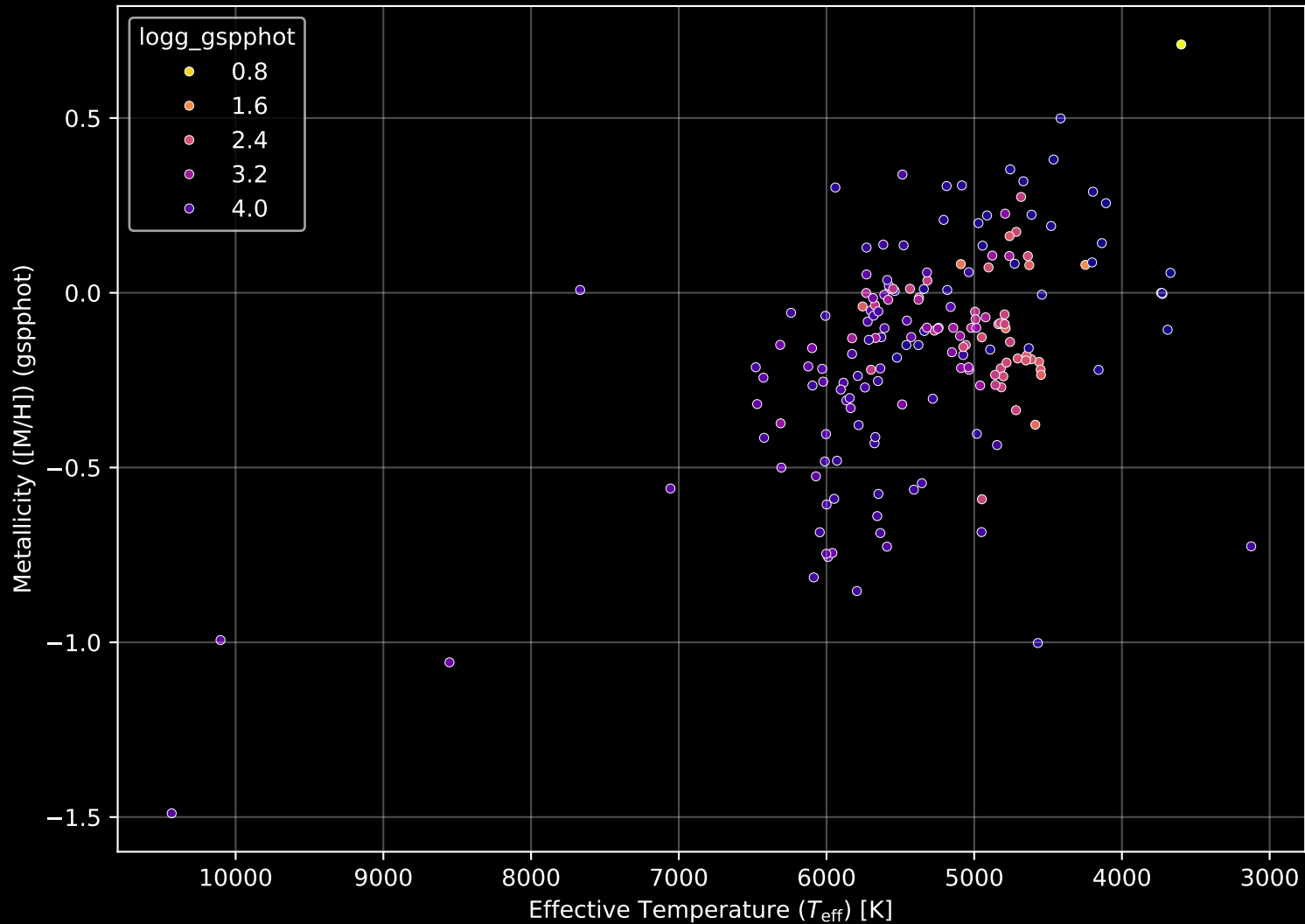
APOGEE DR17 Field: [271-29-O_TESS] Stellar Population Parameters (n= 179)
